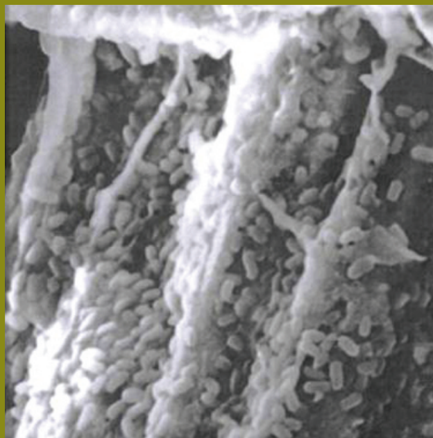
Healthy Bacteria
